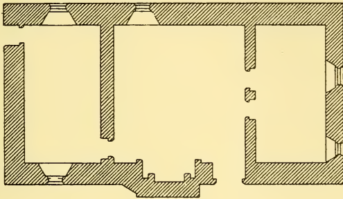
PLAN OF THE FISHING HOUSE AT MEARE.
